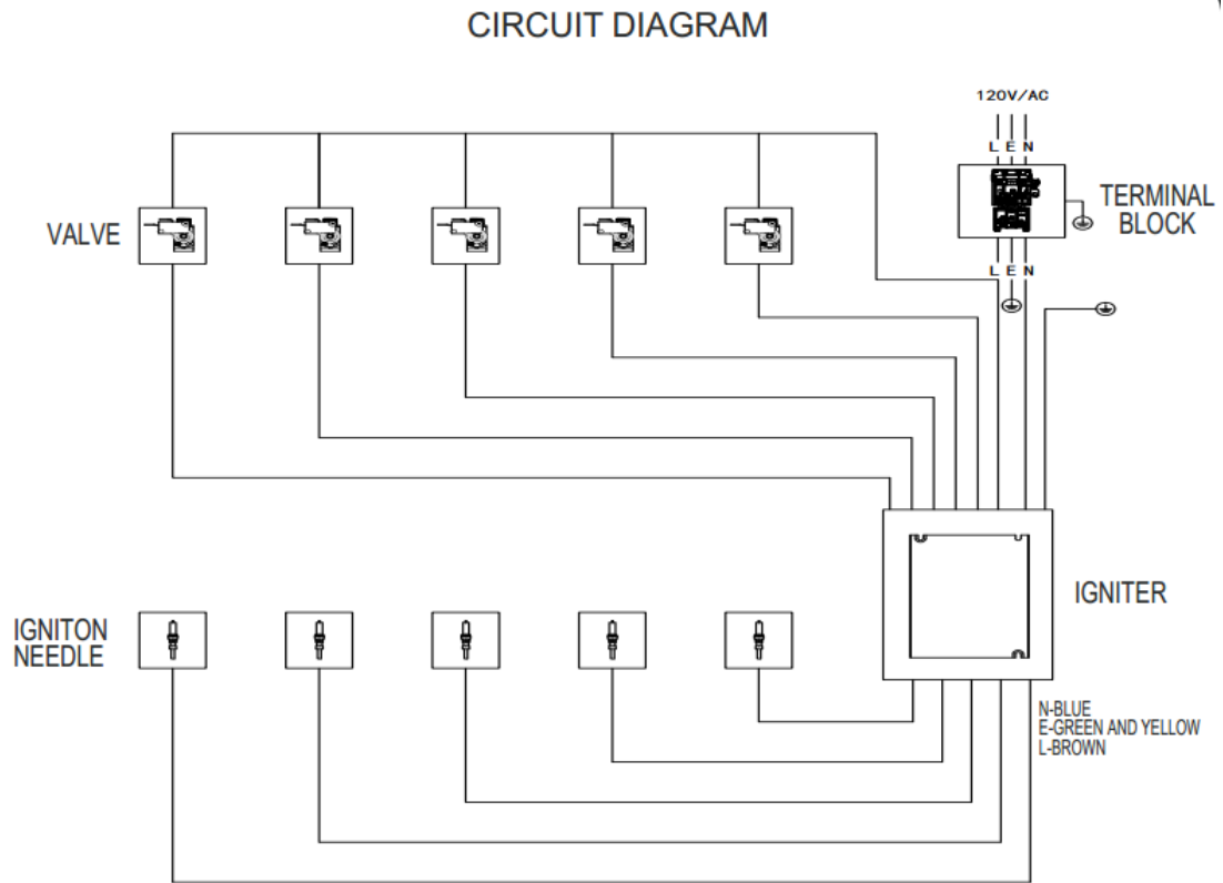
Figure 12(for the appliance with five burners)
