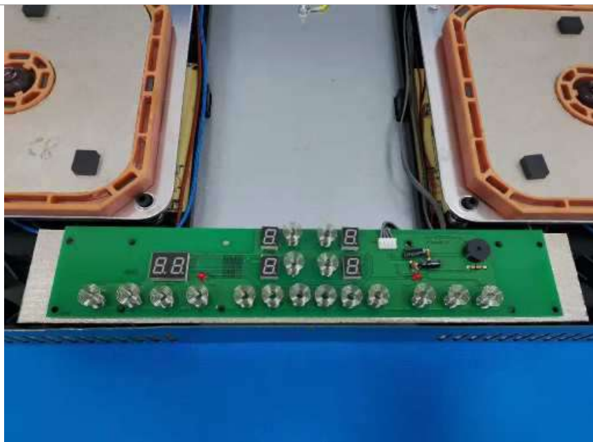
Internal view for GK-IF307204BFF
