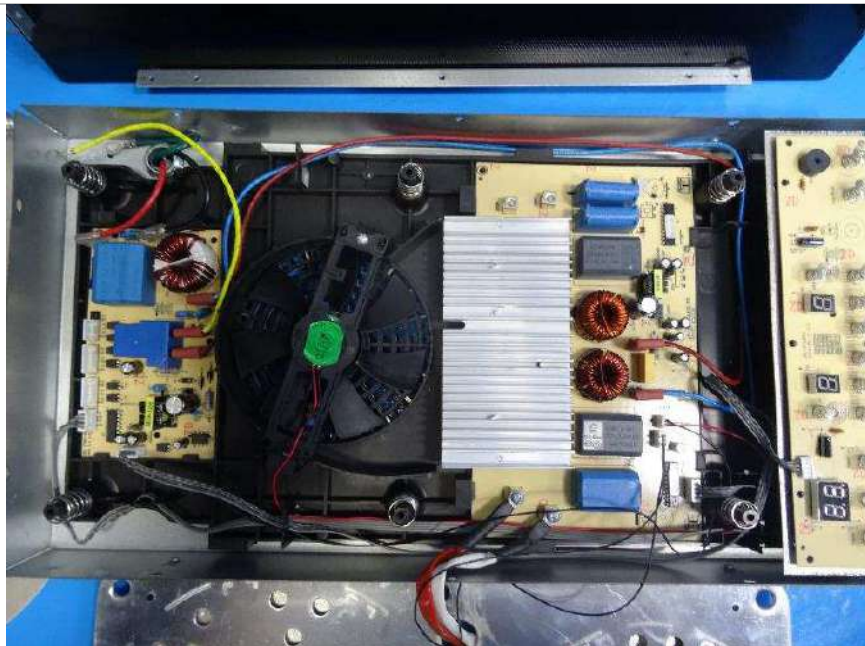
Internal view for GK-ID123604B
