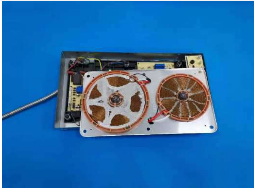
Internal view for GK-ID123604B
