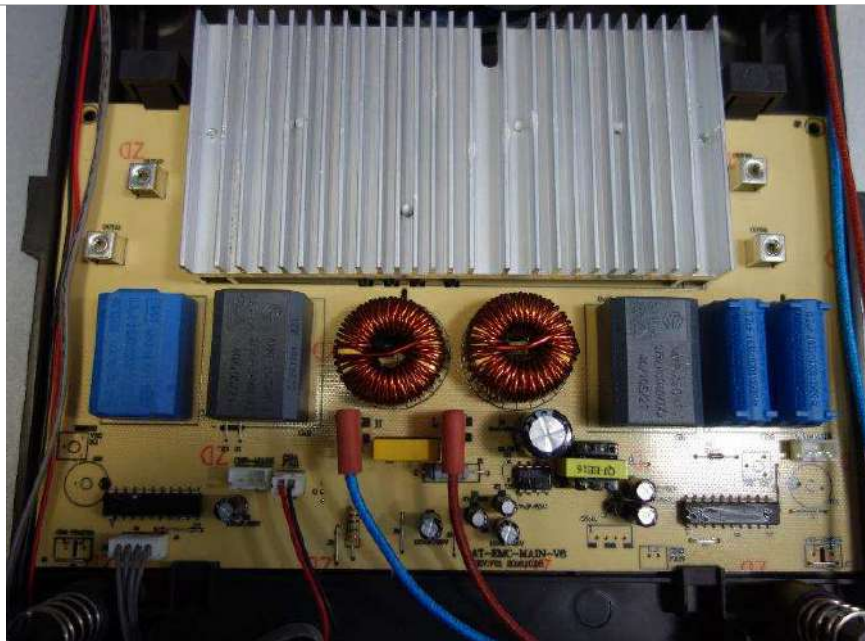
Internal view for GK-IF307209B
