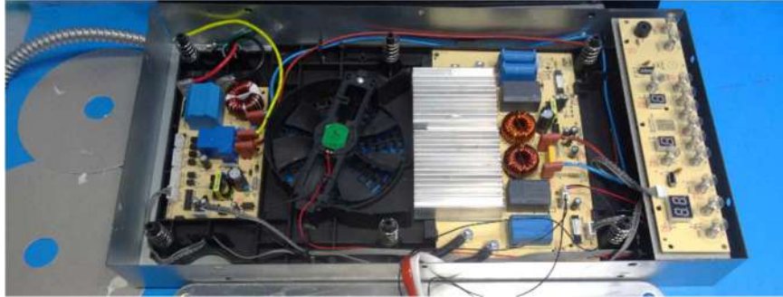
Internal view for GK-ID123604B
